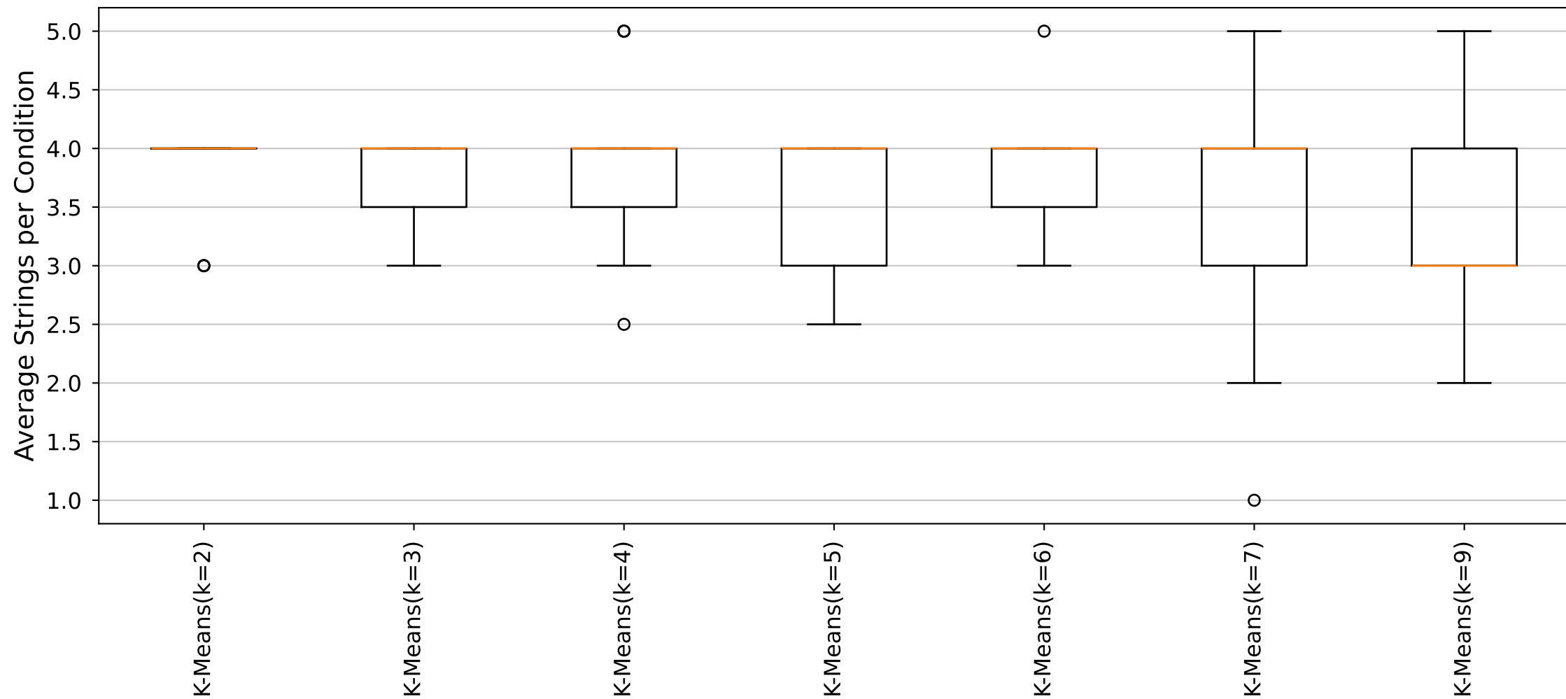
YARA Rules Average Strings per Condition Distribution (Cluster12_Size9 dataset)
